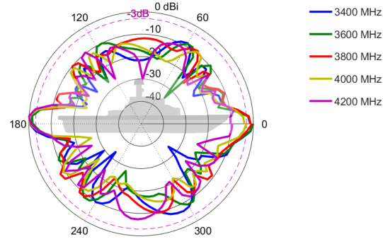
Elevation: 3400 – 4200 MHz
