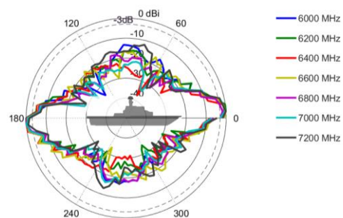
Elevation: 6000 – 7200 MHz
