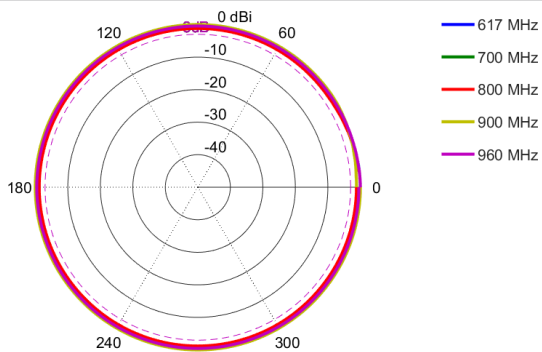
Azimuth: 617 - 960 MHz
