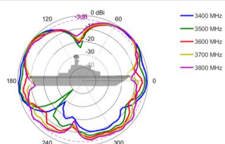
Elevation: 3400 – 3800 MHz
