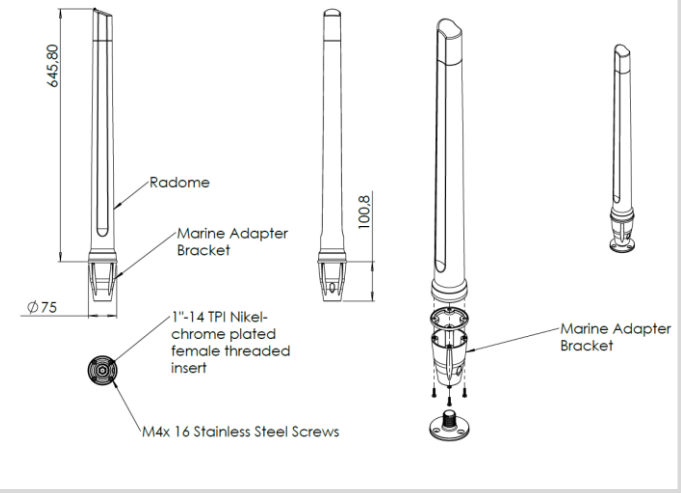
With standard marine mounting
