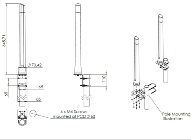
With standard L-bracket mounting
