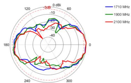
Elevation: 1710 – 2100 MHz
