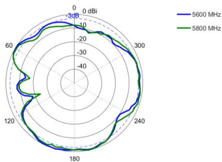
Elevation 2: 5600 – 5800 MHz
