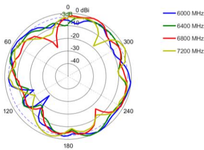
Elevation 1: 6000 – 7200 MHz
