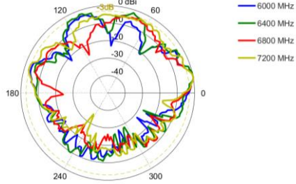
Elevation: 6000 – 7200 MHz
