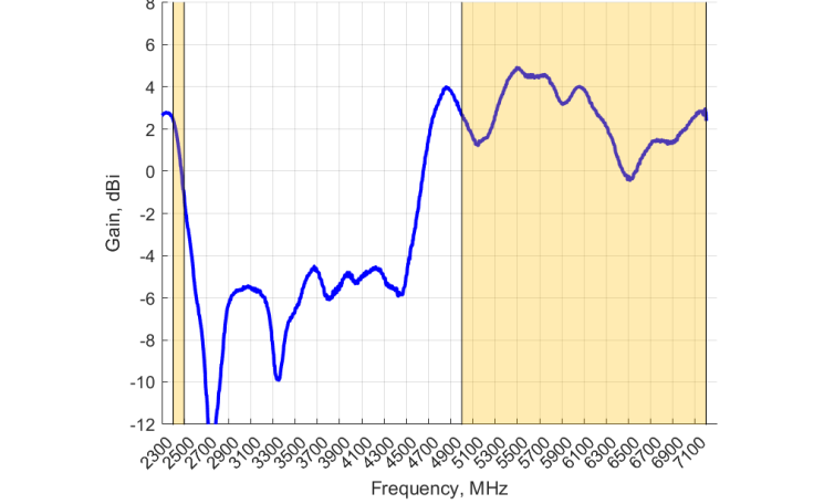
GAIN (Excluding Cable Loss): Wi-Fi Antenna
