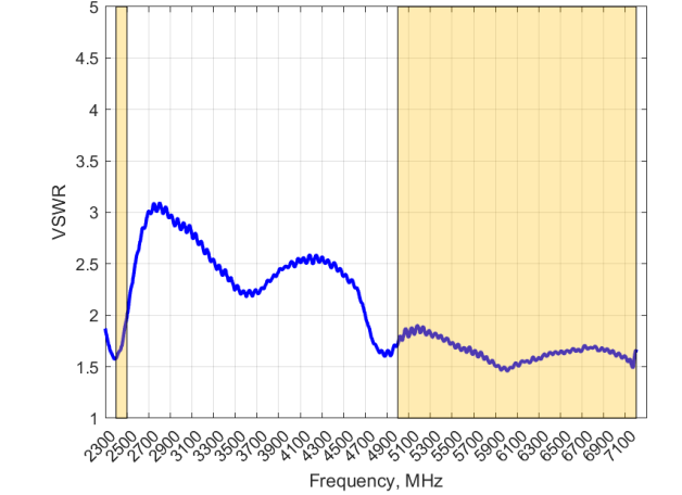
VSWR: Wi-Fi Antenna
