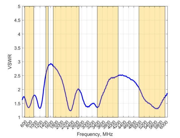
VSWR: Cellular Antenna
