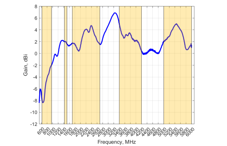
GAIN (Excluding Cable Loss): Cellular Antenna
