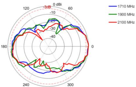
Elevation: 1710 – 2100 MHz
