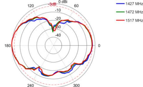
Elevation: 1427 – 1517 MHz
