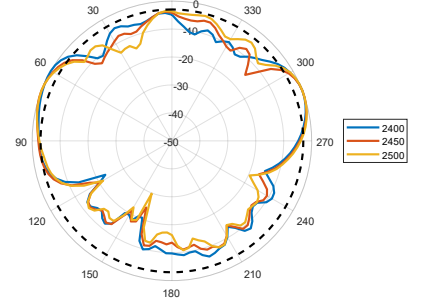
Elevation2 (Side View): 2400–2500 MHz
